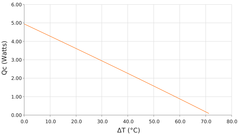
Heat Pumped at Cold Side ( Q_c ) T_{hot} = 35\text{ }^{\circ}\text{C} | operating = 2.1 Amps
