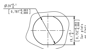
Panel drilling
