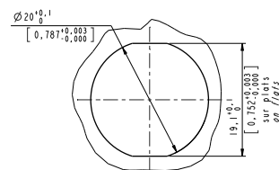
Panel drilling
