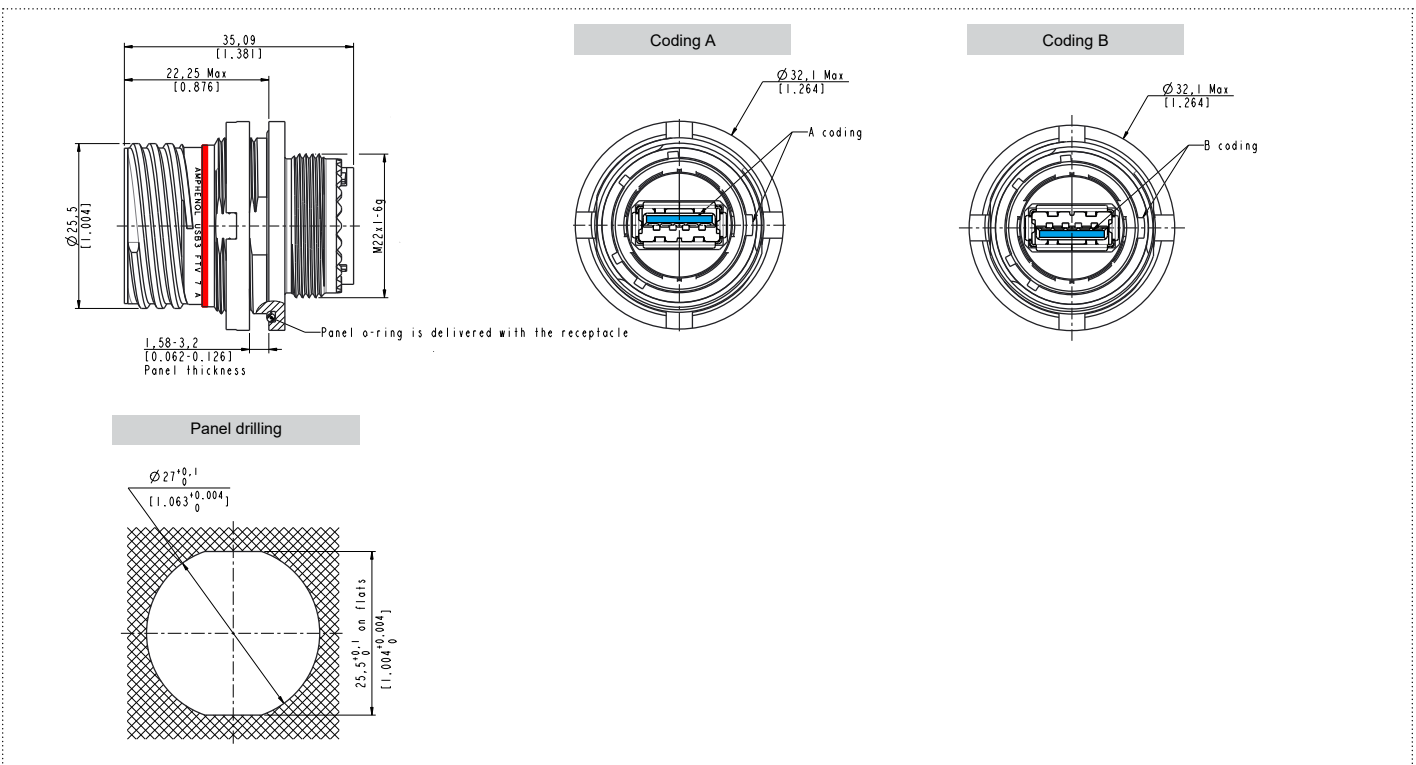
Receptacle - Reduced flange receptacle - Castle nut mounting - Shell type 7 - F312 or F311
