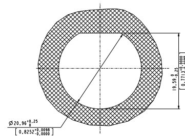
Panel Drilling
