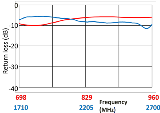
Return Loss
