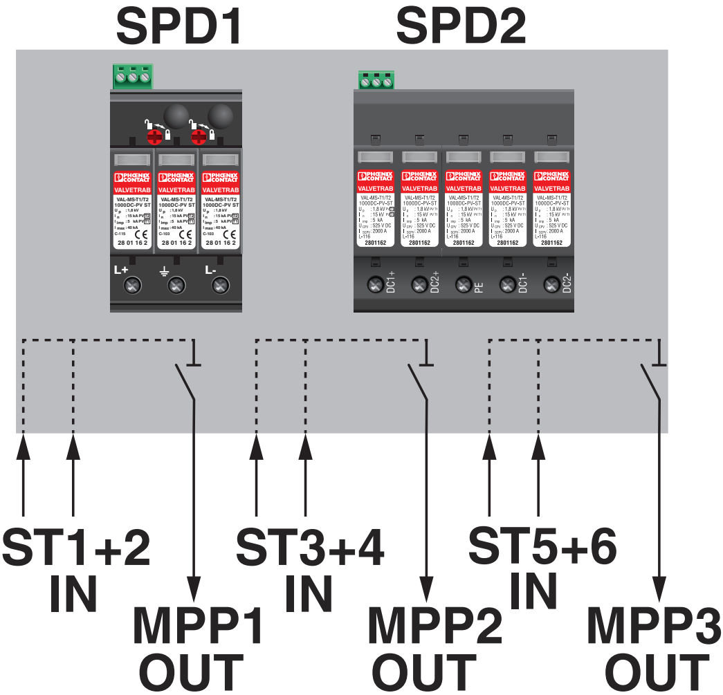
Connection diagram
