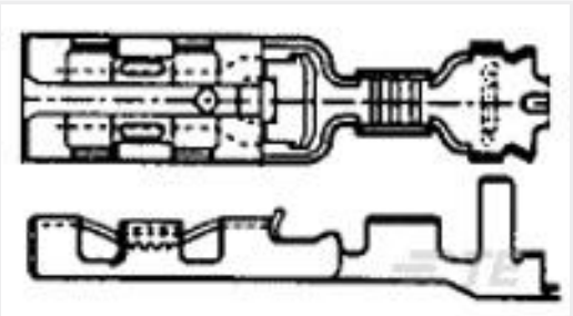
TE Part #1-1565081-2 GRACE INERTIA CONNECTOR 3.5 2P
