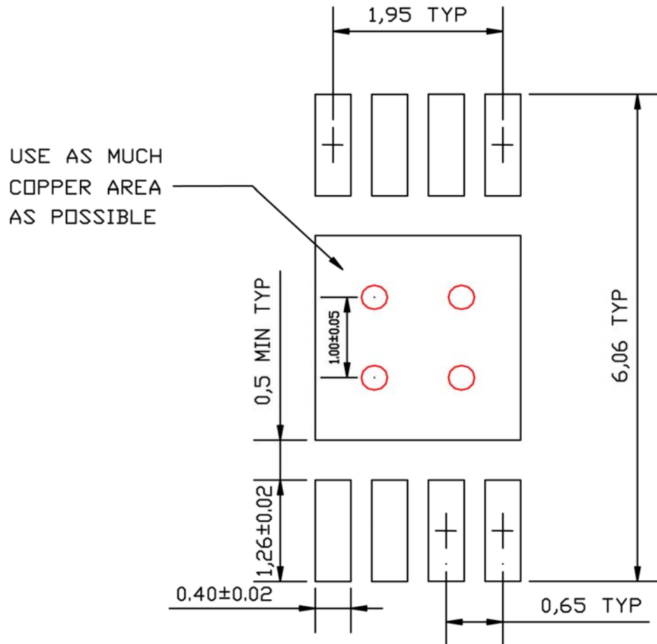
8-Pin Exposed Pad (ePad) MSOP (MME)
