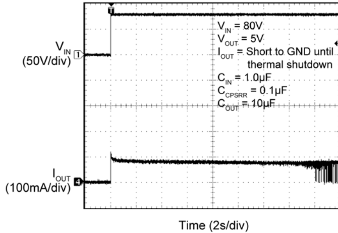
Thermal-Shutdown Response
