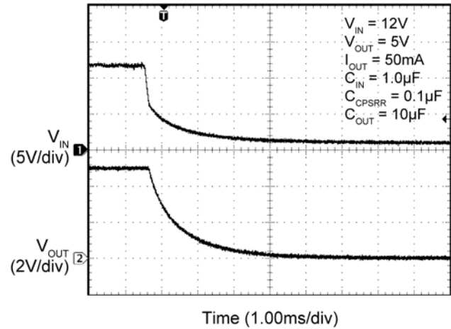
Hot Un-Plug
