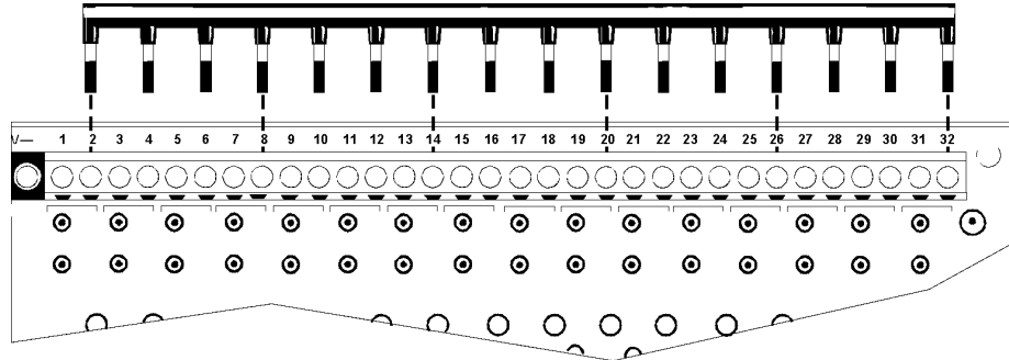
FIGURE 7: G4STRAP USED ON THE G4D32RS
