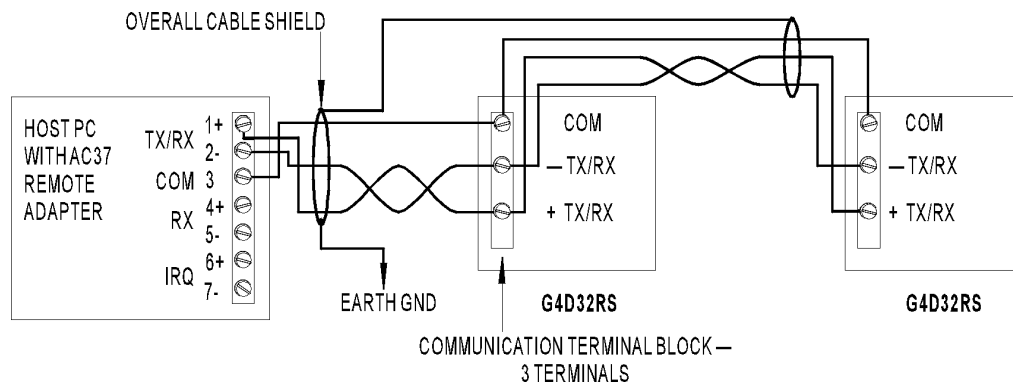
FIGURE 8: TWO-WIRE COMMUNICATION WIRING TO THE G4D32RS I/O UNIT
