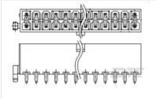
TE Part #1-1775099-3 ATX PWR CONN 1 BDLK 24 POS
