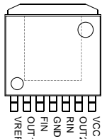
Fig.4 HRP7(TOP VIEW)
