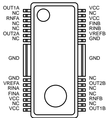
Fig.10 HSOP-M28(TOP VIEW)
