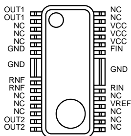
Fig.6 HSOP25(TOP VIEW)
