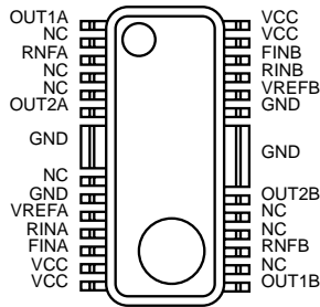
Fig.8 HSOP25(TOP VIEW)
