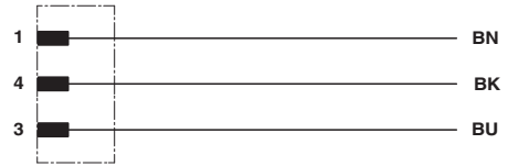
M8 contact assignment
