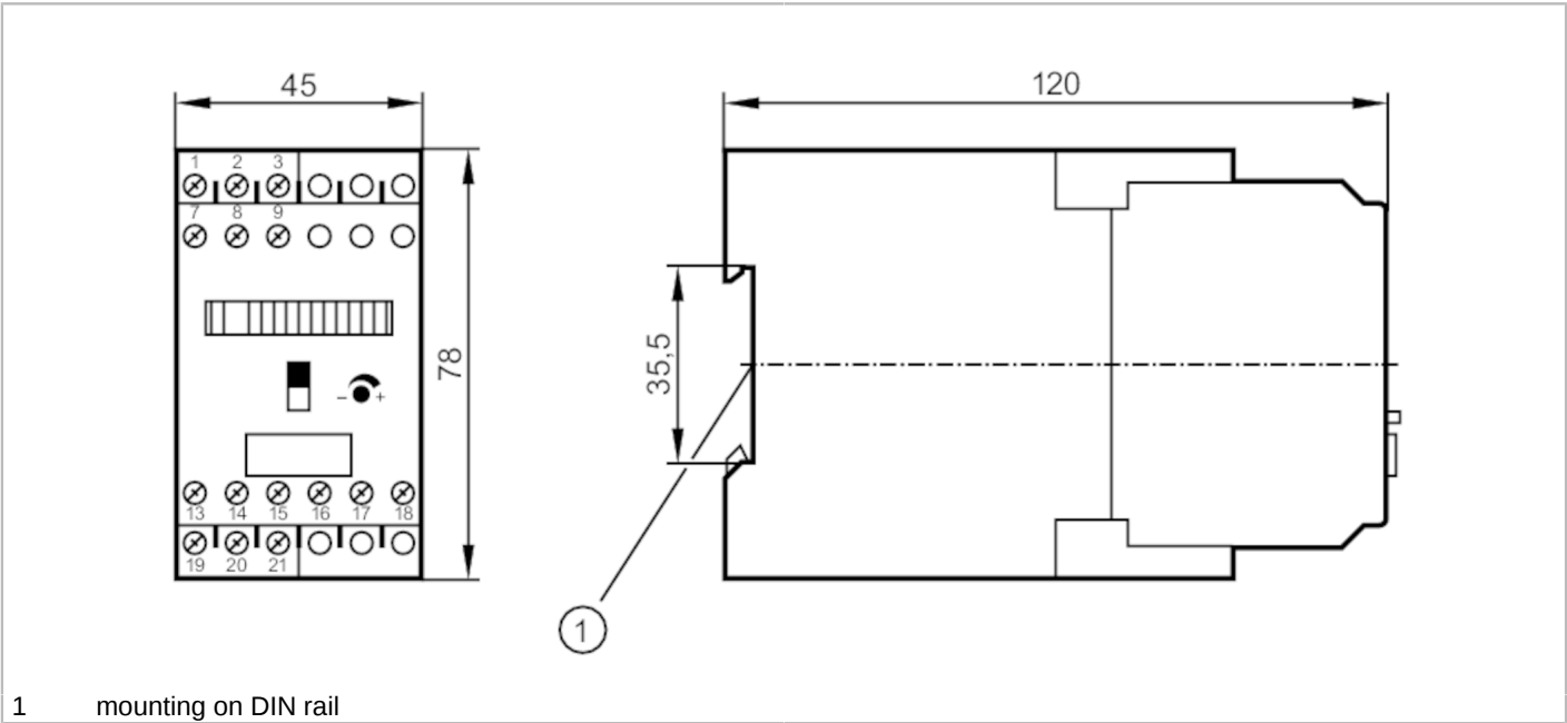
1 mounting on DIN rail
