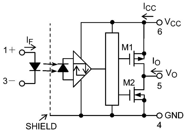
Fig. 5.1 Internal Circuit
