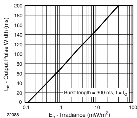
Fig. 8 - Maximum Output Pulse Width vs. Irradiance
