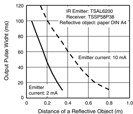
Fig. 14 - Distance Characteristic of a Typical Reflective Sensor using the TSSP58P38
