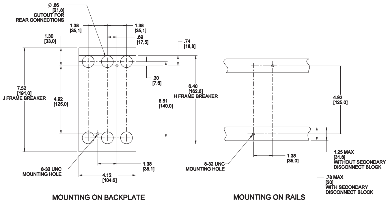
Figure 25: PowerPact H- and J-Frame 3P Circuit Breaker
