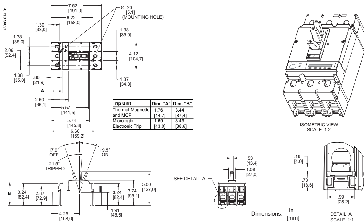
Figure 16: 150–250 A Lug-Lug PowerPact J-Frame 3P Circuit Breaker
