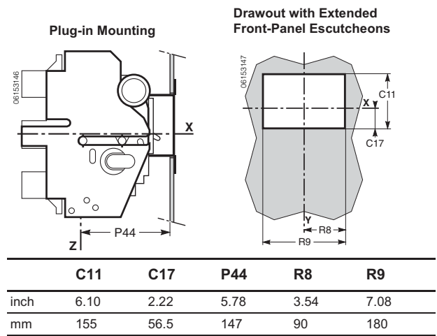
Figure 39: PowerPact L-Frame Circuit Breaker Front-Panel Cutouts
