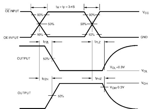
FIGURE 3. AC Waveforms
