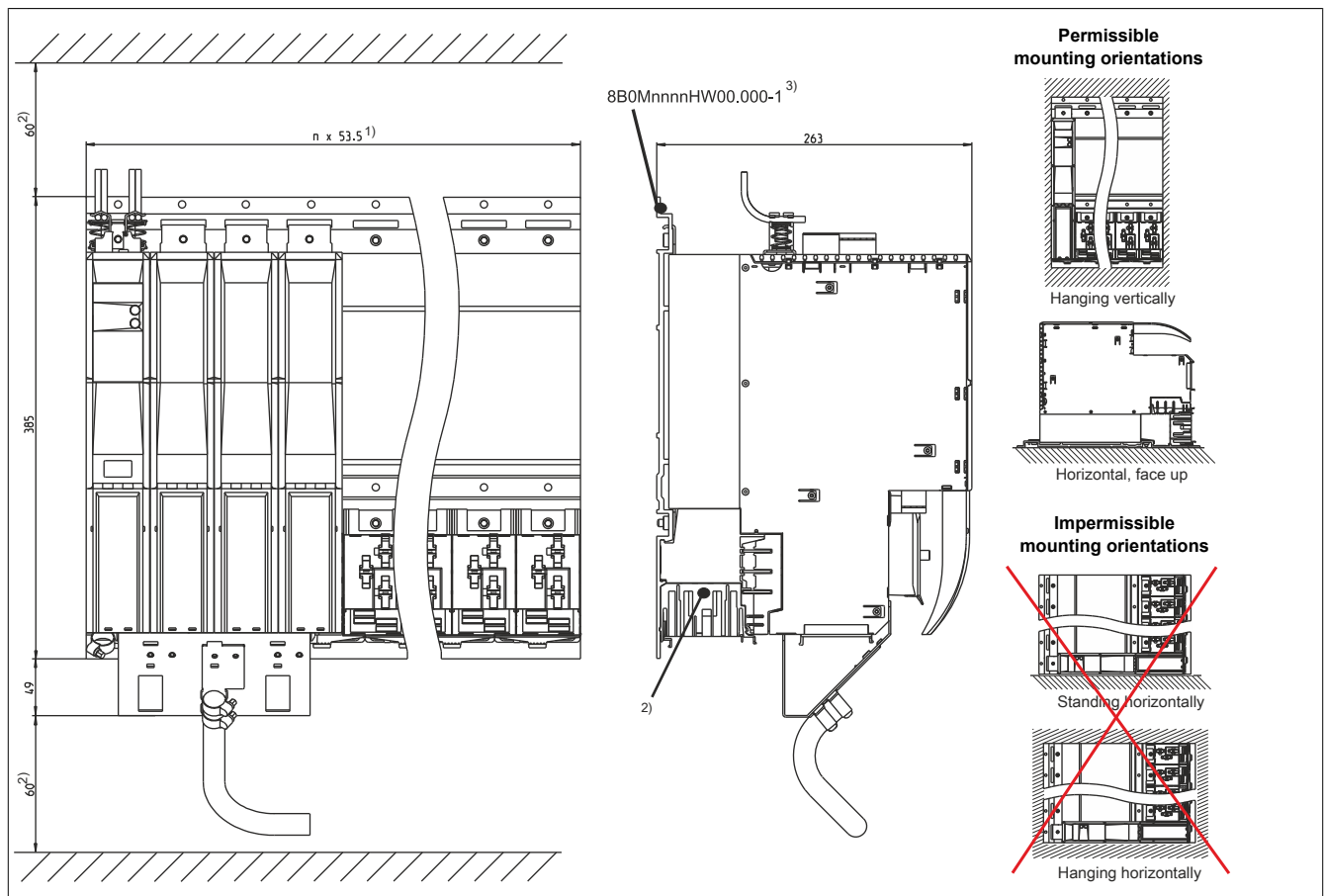
Figure 4: Dimension diagram and installation dimensions
