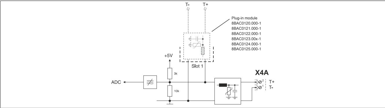
Figure 11: Temperature sensor
