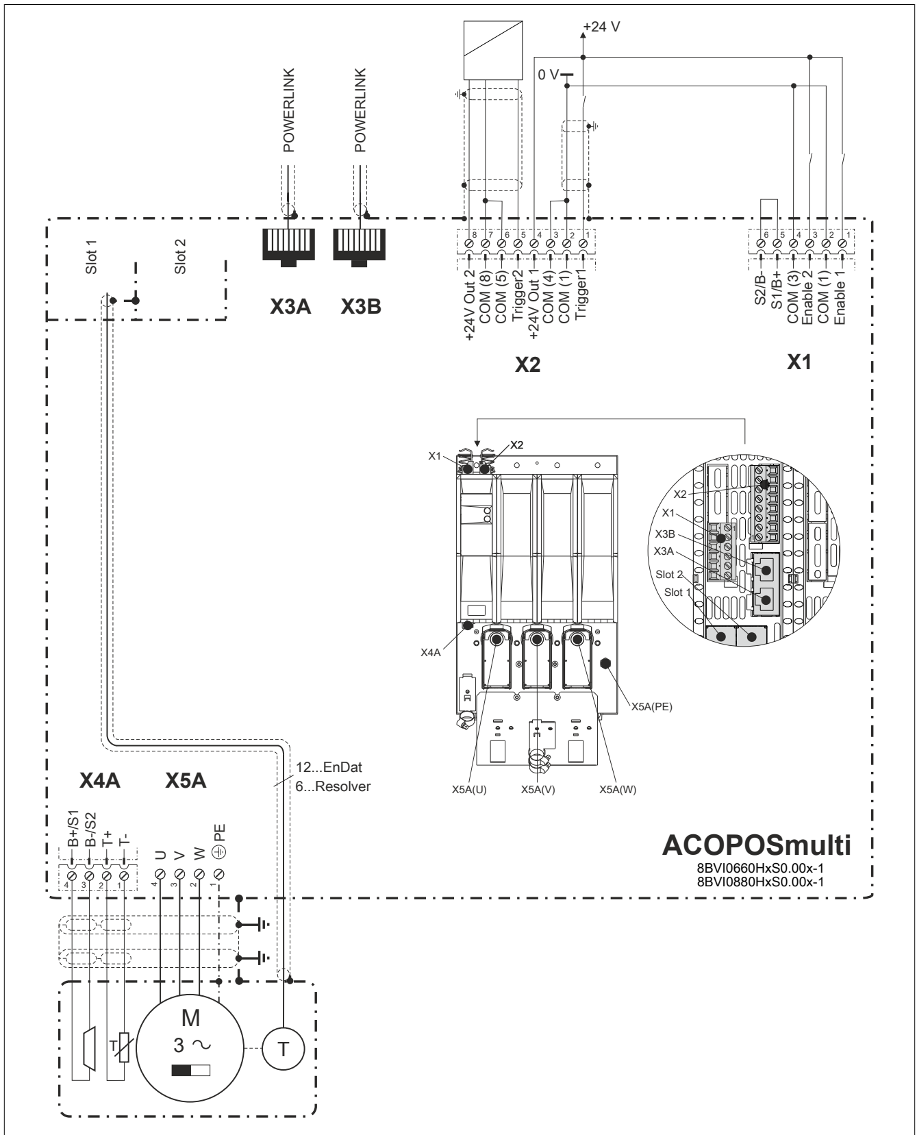
Figure 5: Pinout overview
