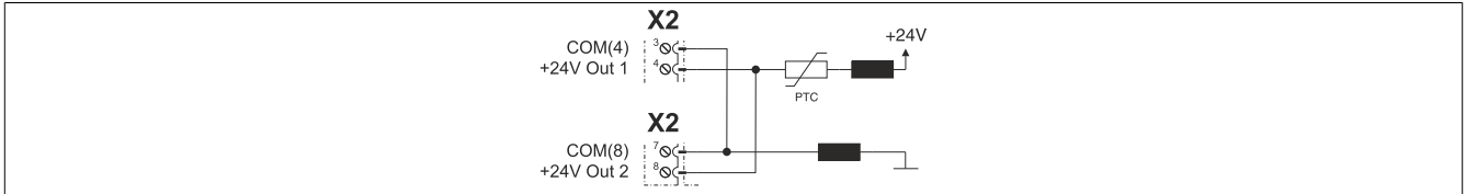
Figure 7: 24 VDC out
