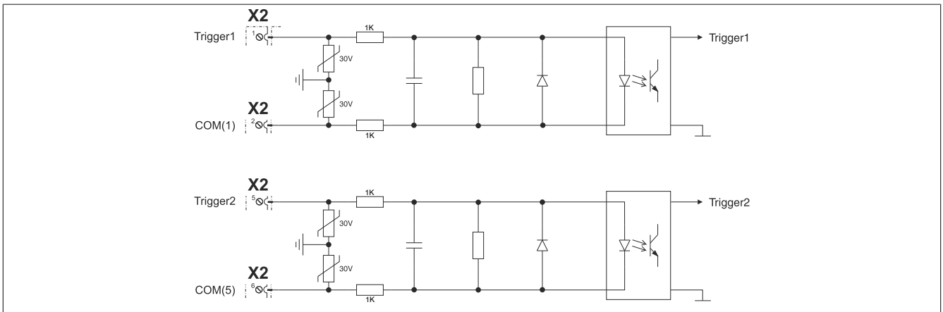
Figure 6: Trigger inputs
