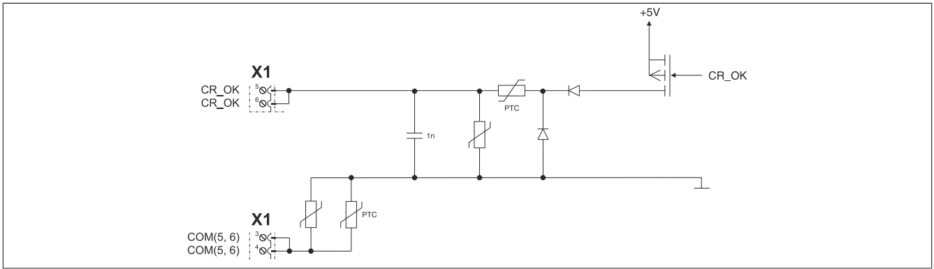
Figure 5: 8B0C - Enable
