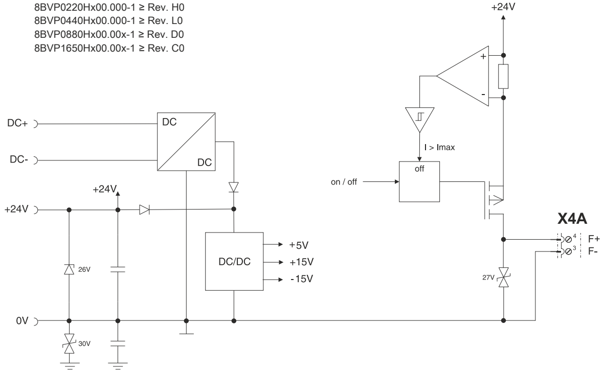
Figure 8: 8BVF fan - Control
