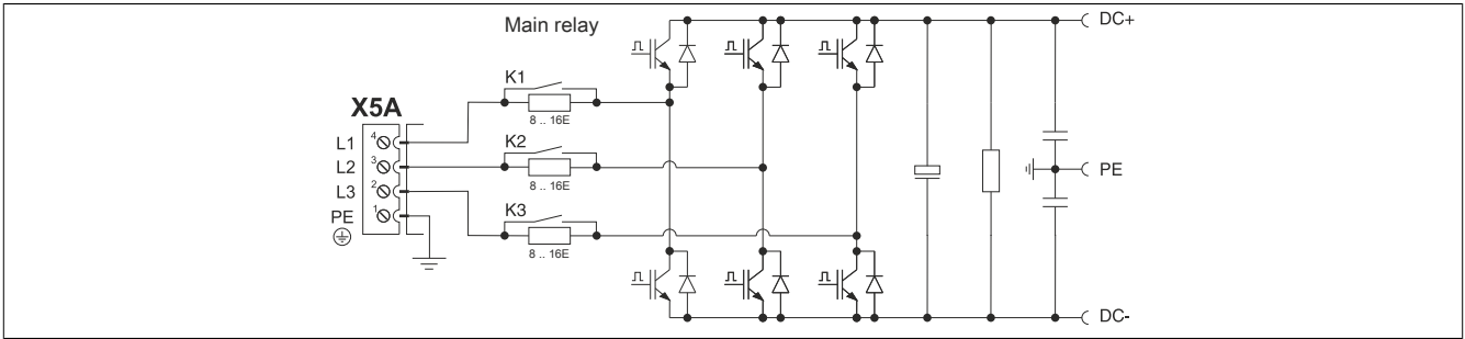
Figure 10: Power unit
