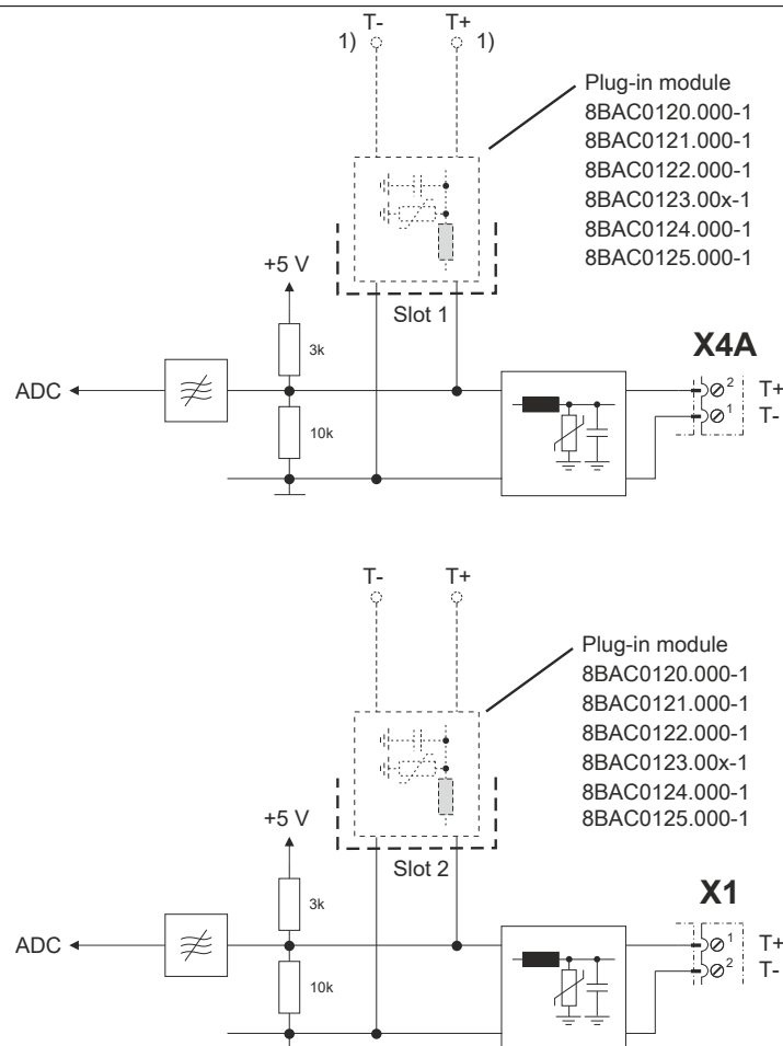
Figure 9: Temperature sensor
