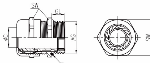
Sealing ring
