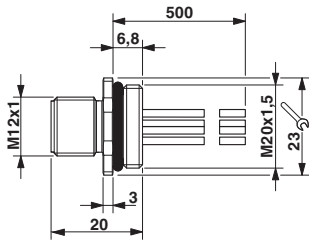
Dimensioned drawing
