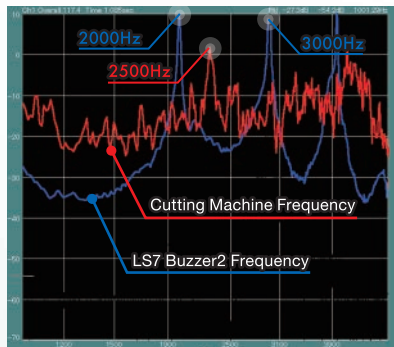
Frequency graph of a metalworking sound and buzzer2 alarm. (Intercompany Measurement) ※ Buzzer1 (Lead Wire or M12 Type) is measured at 2000Hz.
