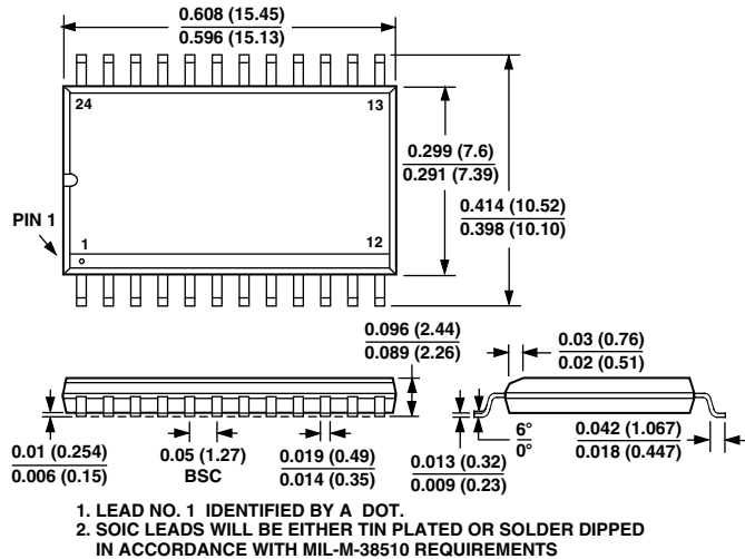
24-Lead SOIC (R-24)
