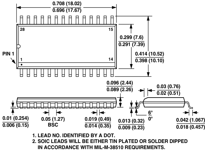
28-Lead SOIC (R-28)
