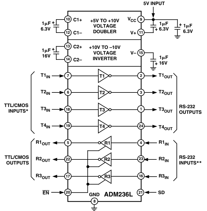
Figure 14. ADM236L Typical Operating Circuit
