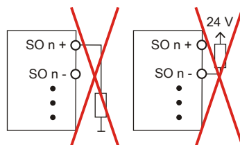
Figure 15: Invalid wiring
