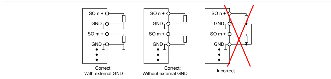
Figure 16: Invalid wiring
