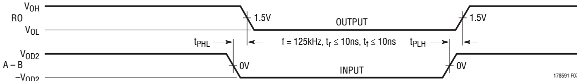
Figure 7. Receiver Propagation Delays
