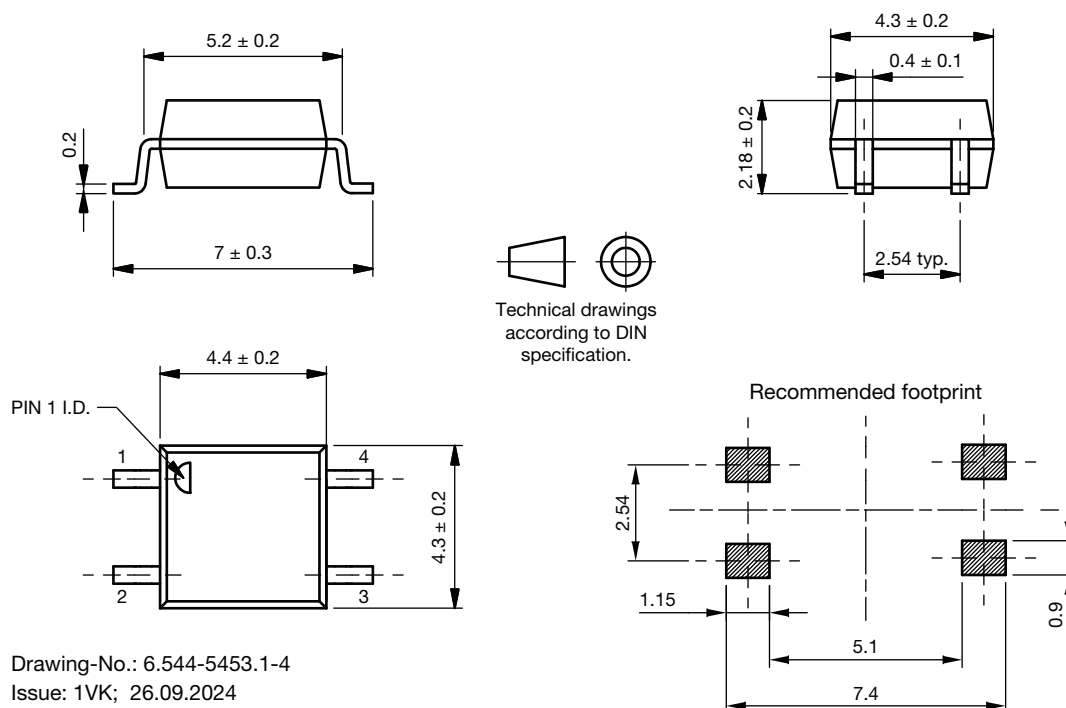
Fig. 14 - Package Drawings
