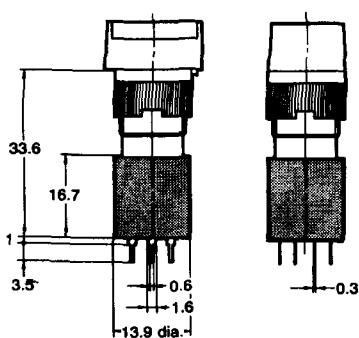
PCB Terminal
