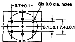
Mounting Hole (Bottom View)
