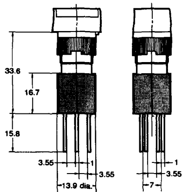
Wire-wrap Terminal
