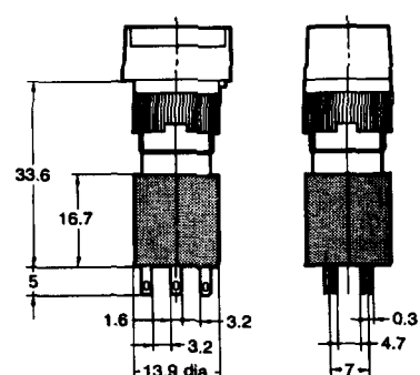
Solder Terminal
