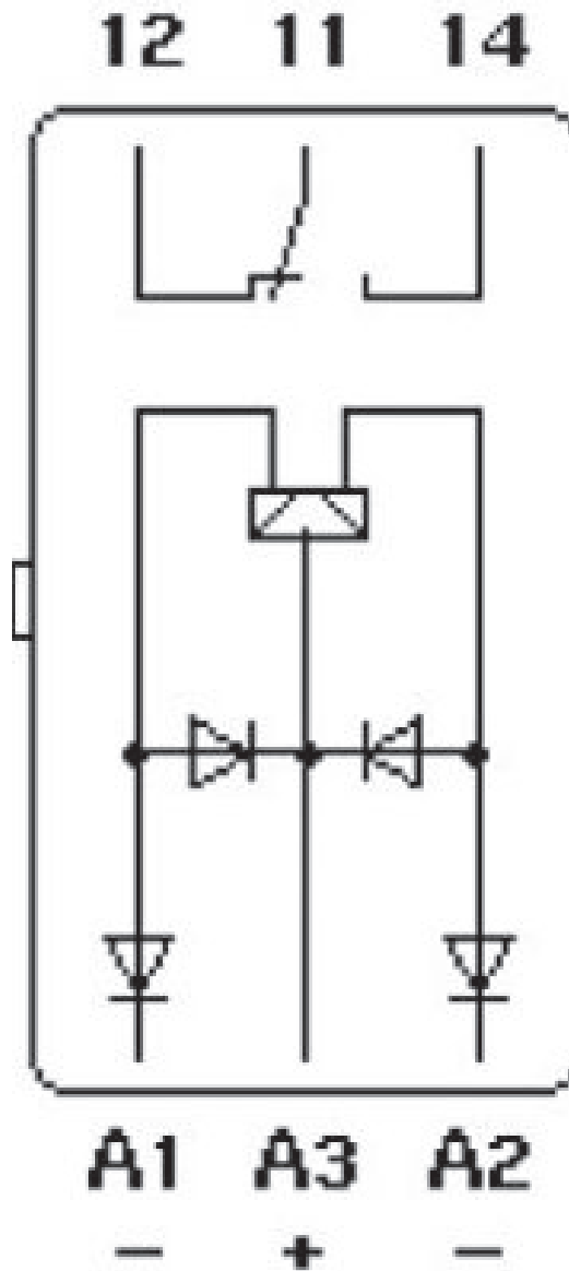
Circuit diagram
