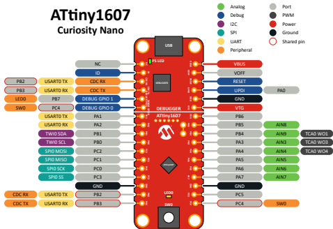
On-Board Peripherals
