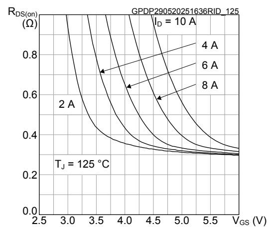
Figure 10. Typical drain-source on-resistance ( T_J = 125 \text{ }^{\circ}\text{C} )
