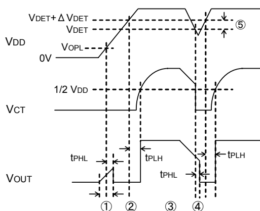
Fig.17 Timing Waveforms
