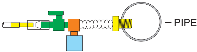
Example 4. Extended ON/OFF Tap Kit
