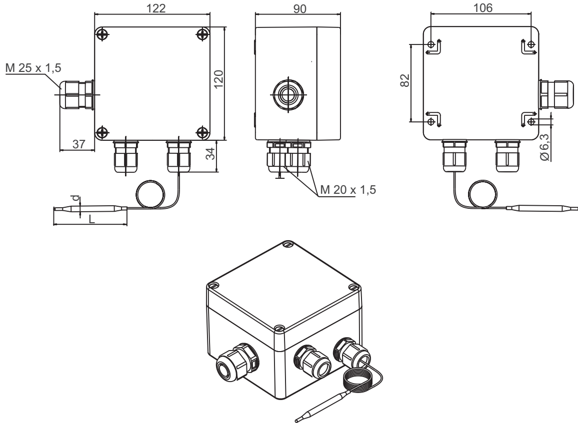
Single thermostat
