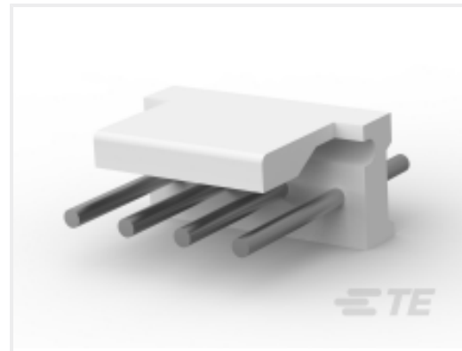
TE Part # 644753-4 04P MTA156 HDR ASSY RN STR F/L
