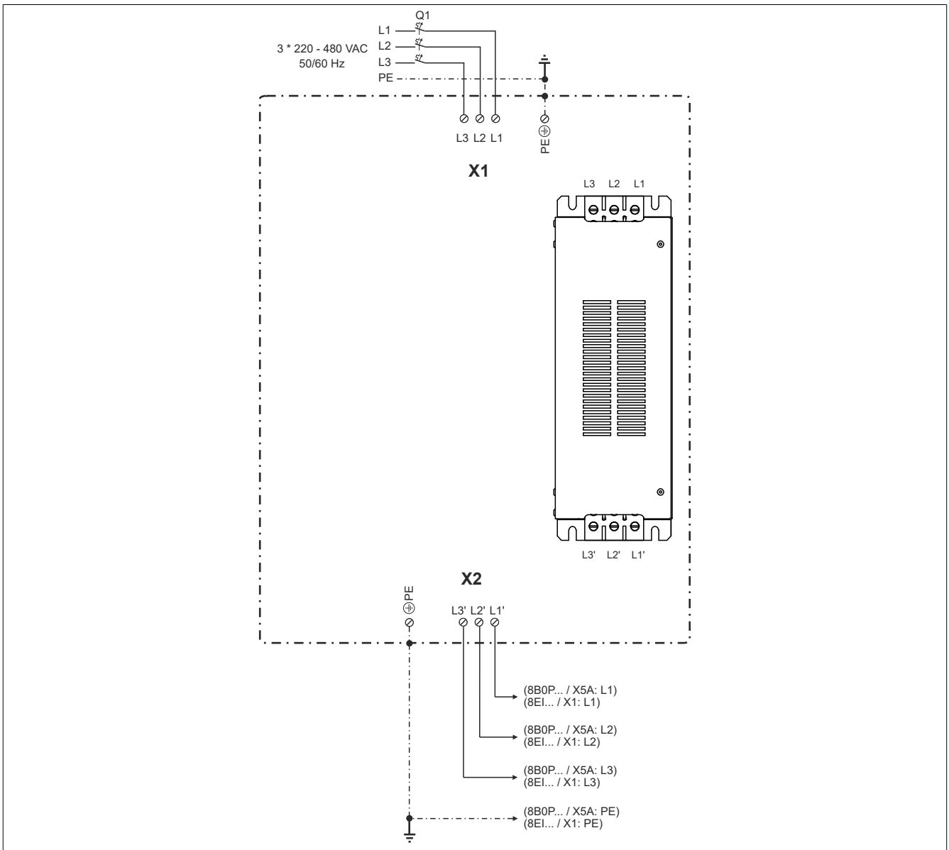
Figure 1: 8B0F0550H000.000-1 - Pinout overview
