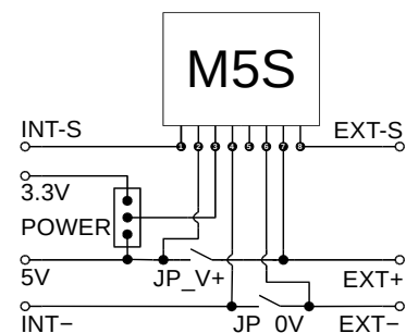
Connection diagram
