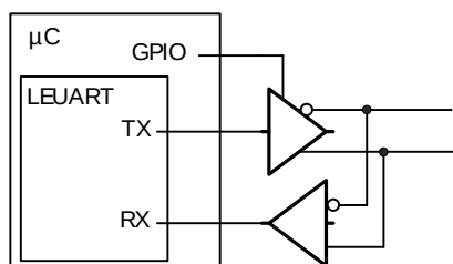
Figure 17.6. LEUART Half Duplex Communication with External Driver
