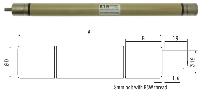
Ferrule fuse links tag type 'A' shown in full lines and '22': tag shown in dotted lines
