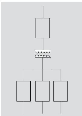
Figure 1 Individual cable exit protection
