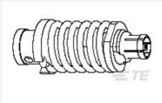
TE Part #1996390-1 SMPM STR CBL JACK
