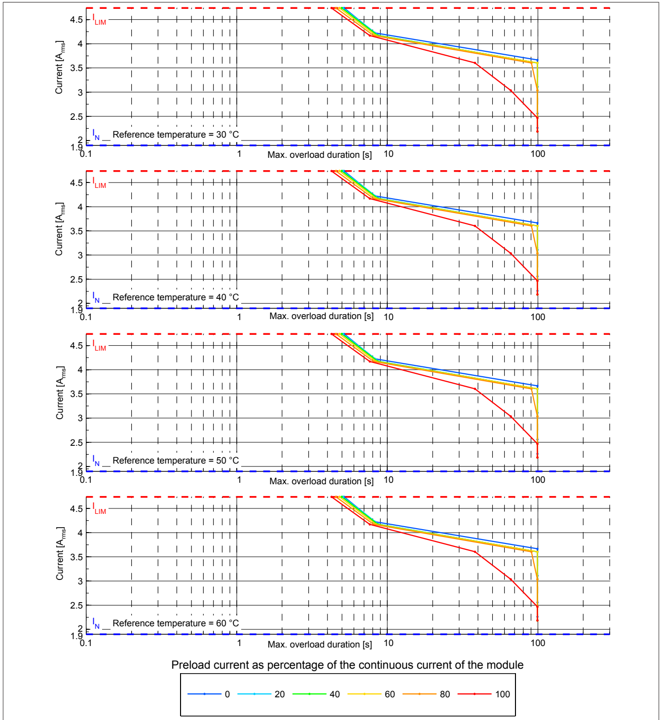
Figure 1: 8BVI0014HCSx.000-x - Overload characteristics, overload response - WARNING
