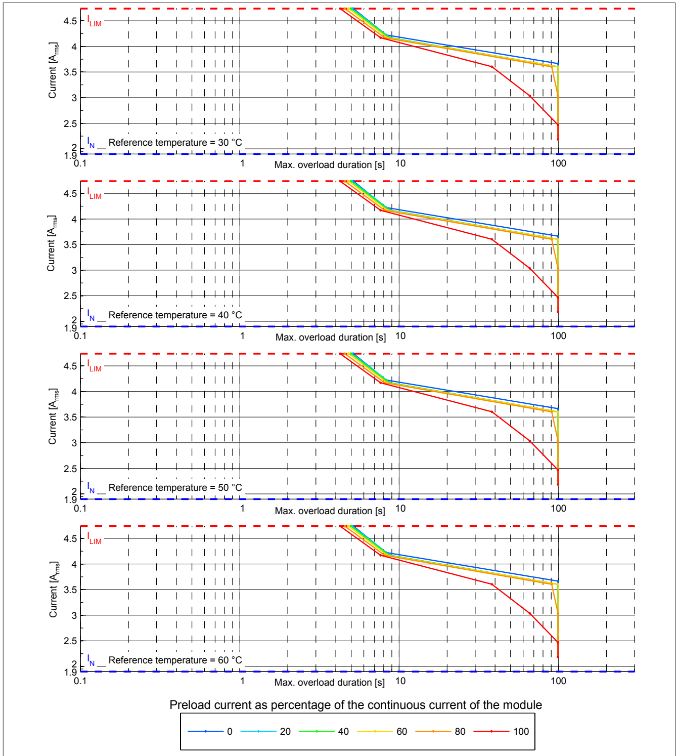
Figure 2: 8BVI0014HCSx.000-x - Overload characteristics, overload response - ERROR+STOP
