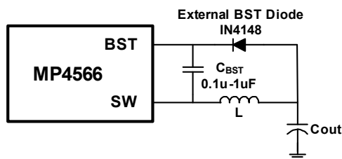
Figure 2—Add Optional External Bootstrap Diode to Enhance Efficiency
