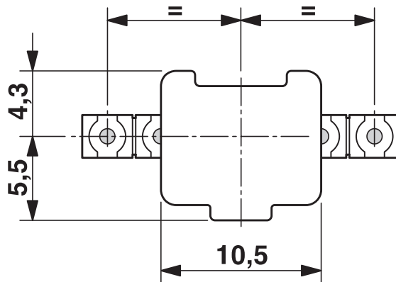
Dimensional drawing
