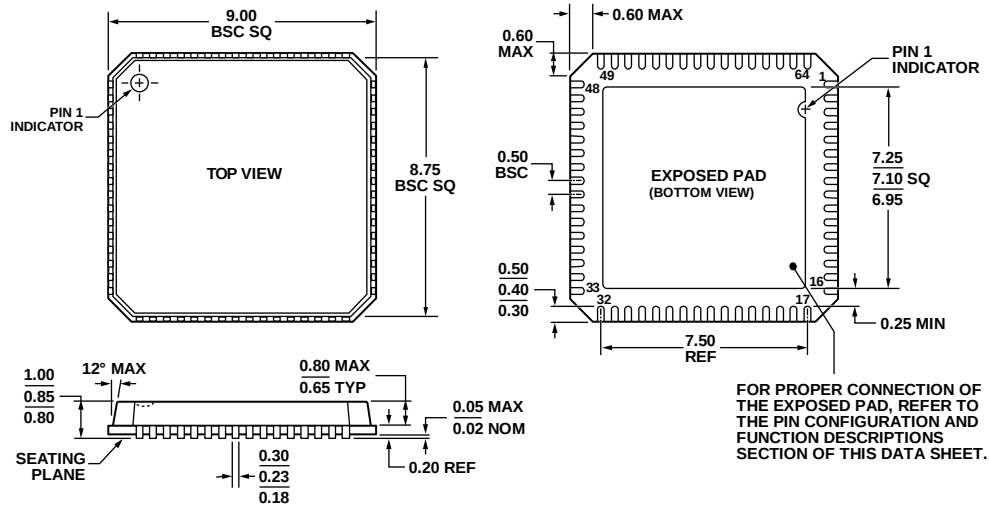
Figure 74. 64-Lead Lead Frame Chip Scale Package [LFCSP_VQ]
