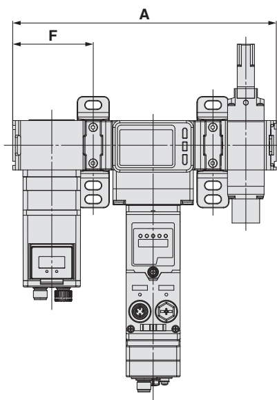
AMS20/30/40/60A-H00C (Sans raccordement)
