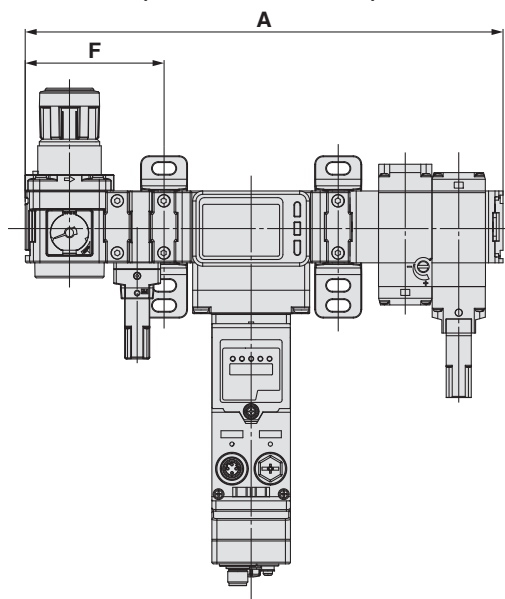
AMS20/30/40/60B-H00D (Sans raccordement)
