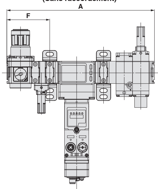
AMS20/30/40/60B-H00C (Sans raccordement)
