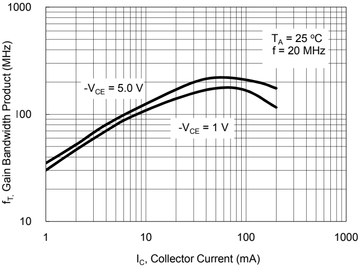
Fig. 2 Gain Bandwidth Product VS. Collector Current
