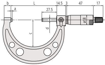
Models up to 75mm
