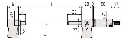
Models over 300mm
