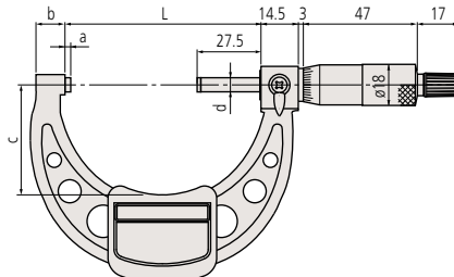
Models 75mm to 300mm
