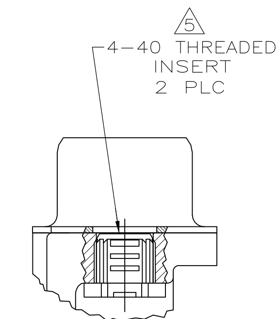
DETAIL D
