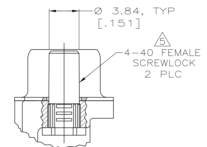
DETAIL E
