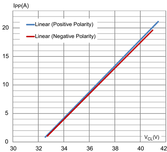
Figure 7. Dynamic resistance
