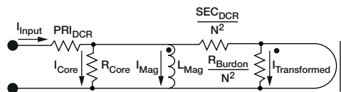
Fig. 2 - Current transformer loss components
