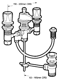
BIDET MIXER WITH POP-UP WASTE (THREE HOLE)
