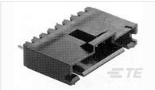
TE Part #5-104363-3 04 MTE HDR SRST LATCH .100CL
