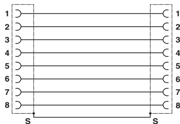
Figure 17 FL-PP-RJ45/RJ45-B (2904933)
