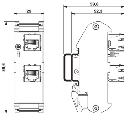
Figure 10 Dimensions FL-PP-RJ45/RJ45
