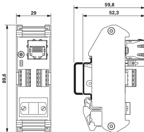
Figure 7 Dimensions FL-PP-RJ45-SC
