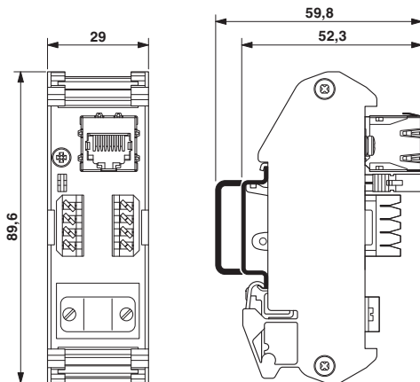
Figure 4 Dimensions FL-PP-RJ45-LSA
