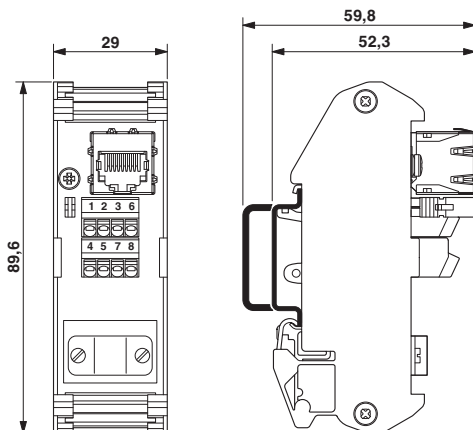
Figure 1 Dimensions FL-PP-RJ45-SCC
