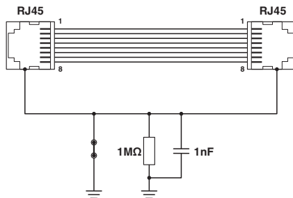
Figure 16 FL-PP-RJ45/RJ45 (2901646)
